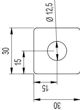
DETAIL REP 6
